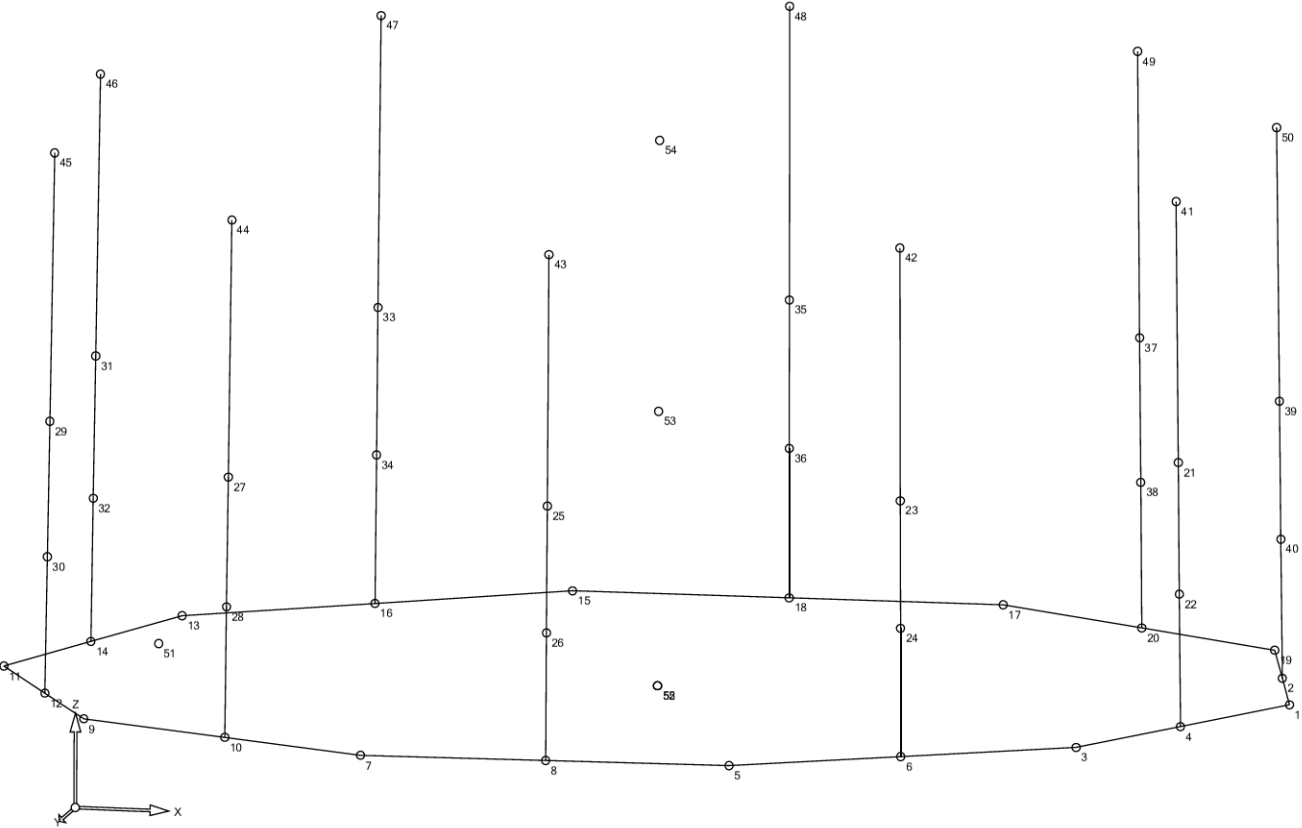
Ring RHS 300x300x10
